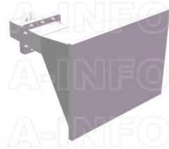
LB-430-15-C-SFSPO Standard Gain Horn Antenna 1.7-2.6GHz 15dB Gain SMA Female
